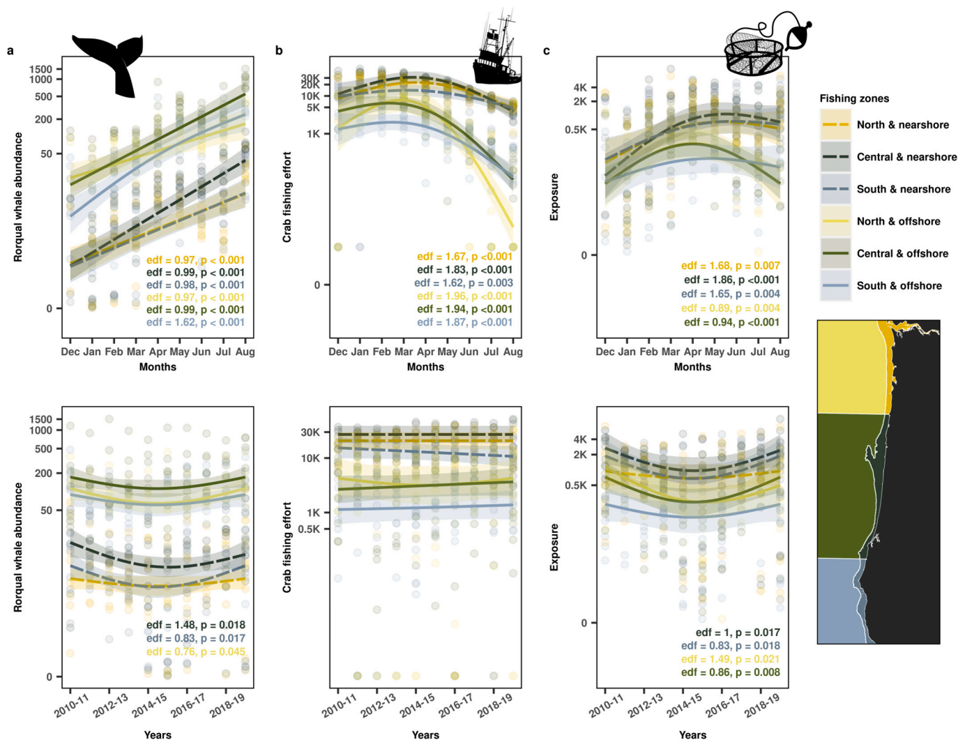
Fig. 2. Fitted relationships between predicted local rorqual whale abundance (a; M_{\text{whale}} ), crab fishing effort (b; M_{\text{crab}} ) and exposure to entanglement risk (c; M_{\text{exposure}} ) with month (top) and fishing year (bottom) predictors. GAMs were fitted to each response type in each of the six study zones represented on the map. Solid and dashed lines represent the marginal effect of month and fishing year by zone, and shaded areas represent approximate 95 % confidence intervals. The estimated degrees of freedom (edf) and the approximate smooth significance of predictors is indicated in each panel when the p-values were below a 0.05 threshold. Data points are represented in light shades. Y-axes are presented on a log scale.
